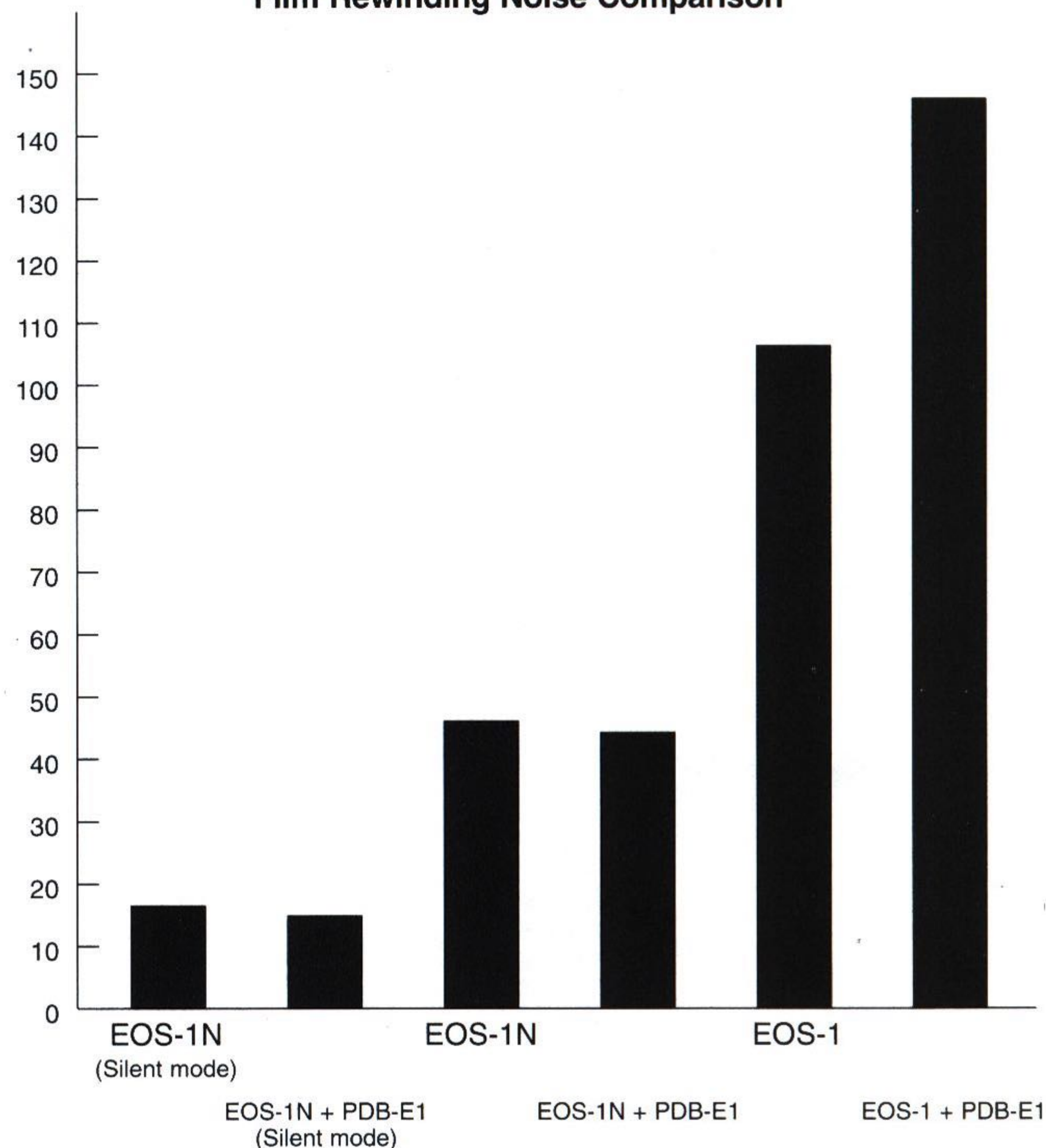
Film Rewinding Noise Comparison
