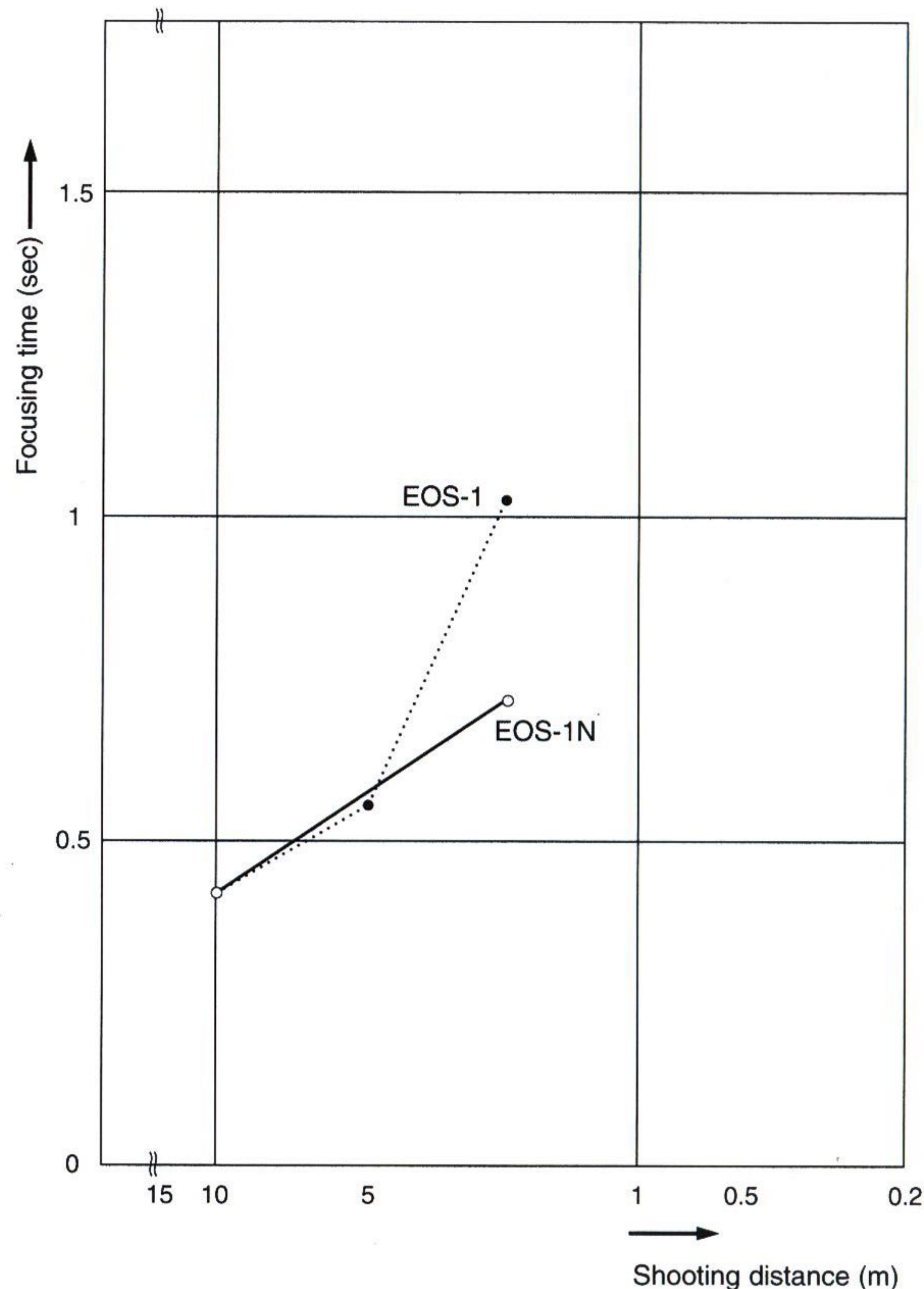
AF focusing speed using the EF300mm f/2.8L USM
