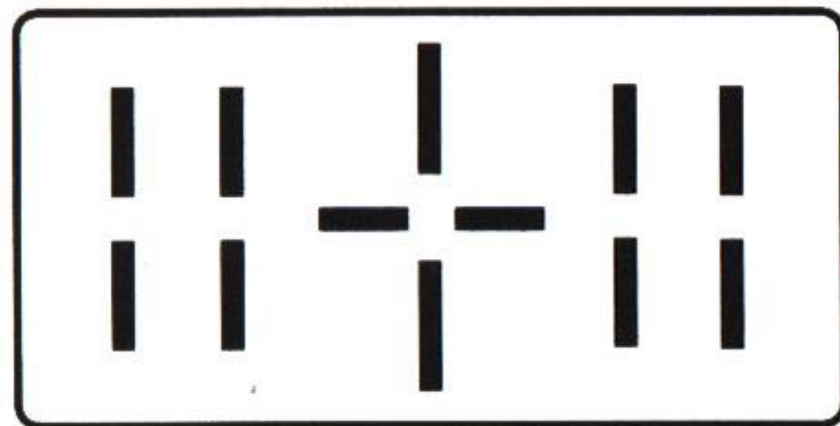
EOS A2/A2E BASIS Sensor Layout
