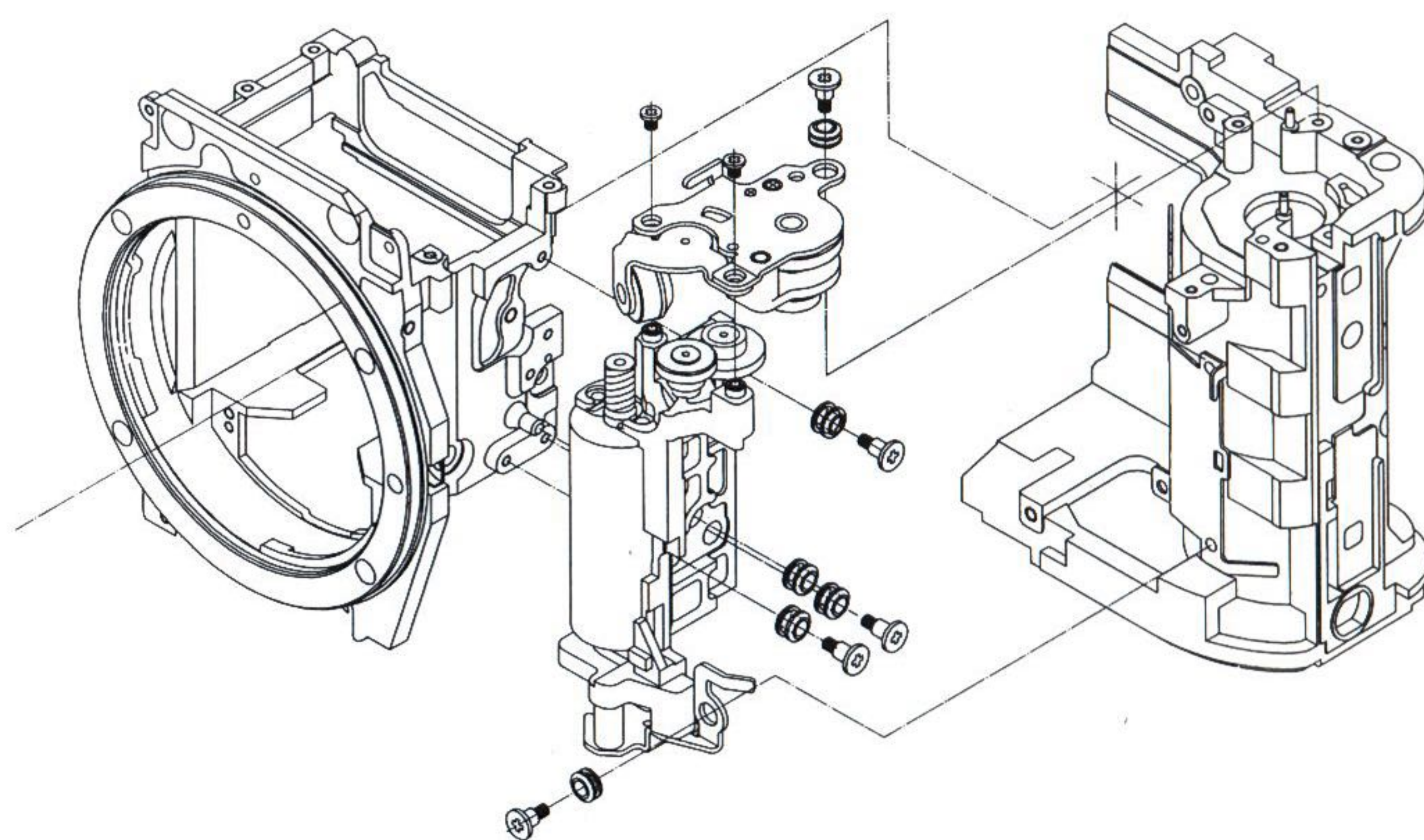
EOS-1N Rewinding System
